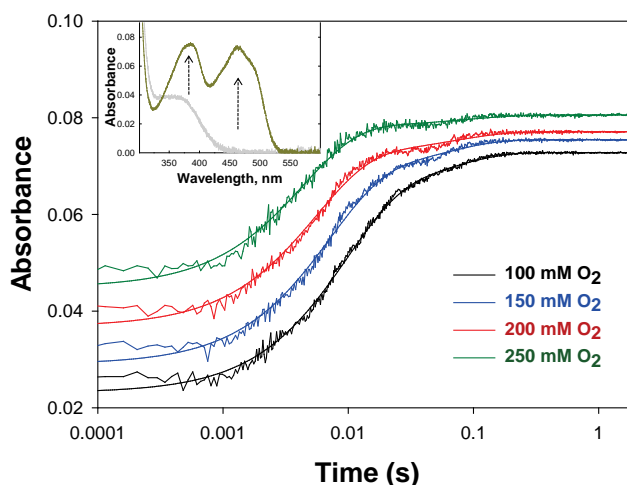
Figure 2. Time-resolved absorbance spectroscopy of the oxidation of reduced AAO at varying O 2 concentrations. The anaerobic enzyme was premixed with [ \alpha - 1 H 2 ]- p -methoxybenzyl alcohol (0.9-fold the enzyme's concentration), allowed to age for 1 s and the reduced enzyme finally mixed with buffers containing various O 2 concentrations (shown in legend). Traces at 463 nm show the two phases of the reaction, fast and slow. Solid line indicates the fit of the traces to a double-exponential process. Inset displays spectra of the initial (reduced, grey) and final (oxidized, dark yellow) flavin species, with arrows indicating the direction of the spectral changes. Conditions: enzyme (5 \mu\text{M} after double mixing) in 100 mM sodium phosphate, pH 5.0, and 12°C.
