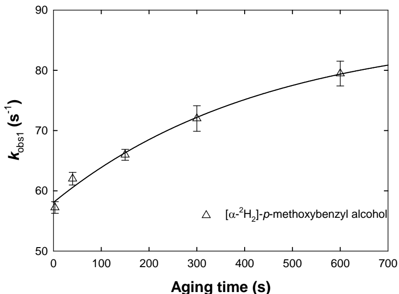
Figure 5. Deuterium wash-out from flavin N5 by exchange with protons from the protiated buffer. k_{obs} dependence on the incubation time of the enzyme labeled with D at the N5 in H 2 O buffer. AAO was premixed and incubated with [ \alpha - 2 H 2 ]- p -methoxybenzyl alcohol (0.9-fold the enzyme's concentration) for various aging times (3–600 s), after which the reduced enzyme was mixed with 136 \mu M O 2 . Conditions: Enzyme (5 \mu M after double mixing) in 50 mM sodium phosphate, pH 6.0, at 12°C. k_{obs} values and standard deviations were estimated from triplicates and fitted to an exponential equation that yielded y = 28.7 \times (1 - e^{-0.0023t}) + 58.1 ( R^2 = 0.989 ).
