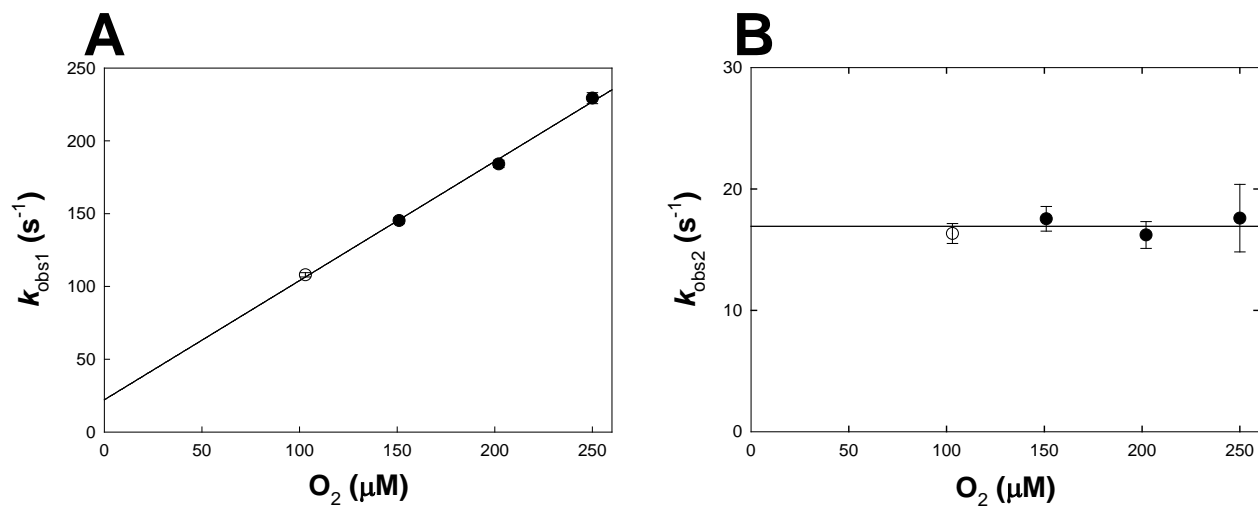
Figure 3. Plot of the observed rate constants ( k_{\text{obs}} ) for the fast ( k_{\text{obs1}} ; A ) and slow ( k_{\text{obs2}} ; B ) phases of AAO oxidation as a function of O_2 concentration. The anaerobic enzyme was premixed with [ \alpha\text{-}^1\text{H}_2 ]- p -methoxybenzyl alcohol (0.9-fold the enzyme's concentration) until complete reduction, and then mixed with varying O_2 concentrations (100–
