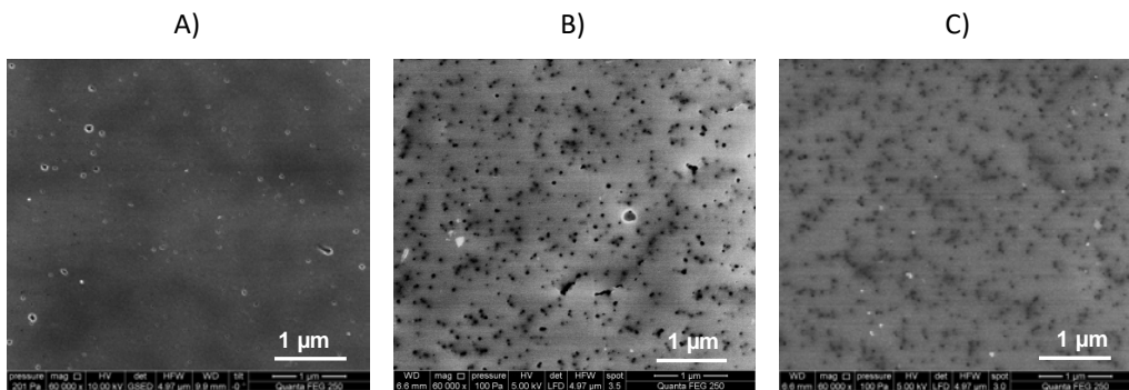
Figure 3. Top view of nanoporous TE PBI membranes: A) PBI_30_0.7; B) PBI_30_3.5; B) PBI_50_10
