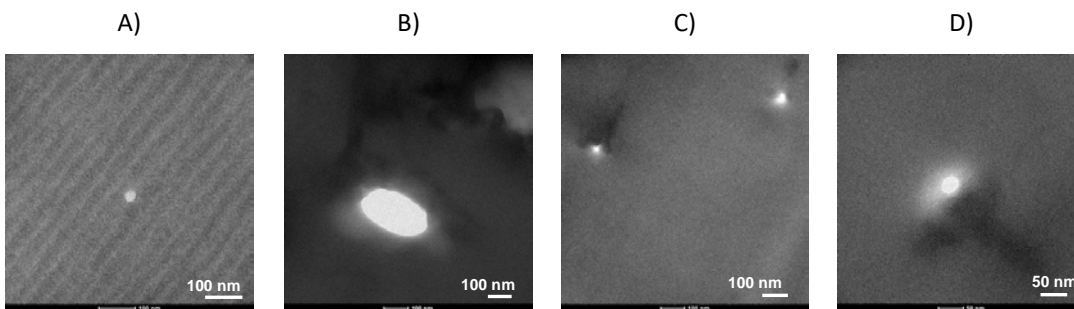
Figure 4. TEM analyses of pore size variation with the depth in the PBI_30_0.7 sample: A) top surface, B) 10 \mu\text{m} to the top surface; and the PBI_15_0.7 sample: C) top surface, D) 10 \mu\text{m} to the top surface.
