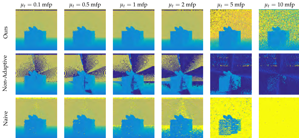
Fig. 4. Recovered depth maps for increasing media densities [from left to right \mu_t = (0.0213, 0.1064, 0.2128, 0.4255, 1.0638, 2.1277) m^{-1} ], with our method (top), the non-adaptive transient PDI method (middle), and the naive unpolarized approach (bottom). The ground truth depth map can be found in Fig. 3, while Fig. 5 shows the mean absolute error for each image.
