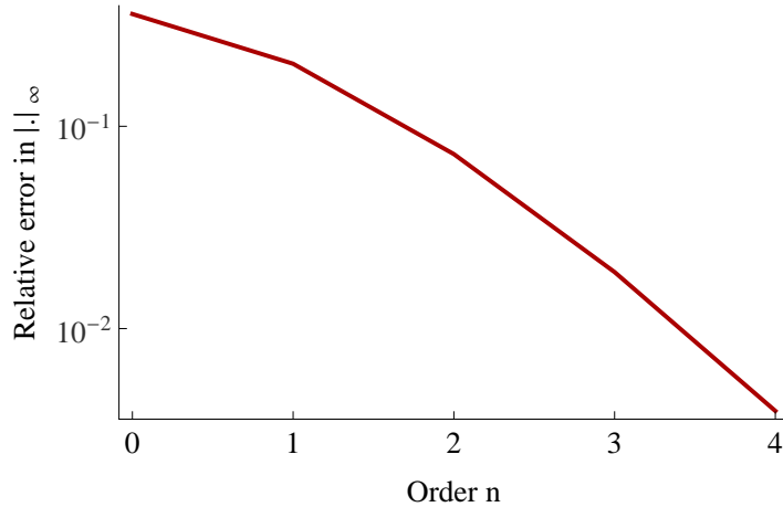
Figure 4: Relative errors in the supremum norm for problem (31) with C = 0 , a = b = \tilde{c} = \tilde{d} = 1 , c = d = \tilde{a} = \tilde{b} = 0 , \alpha = \beta = 1 .
