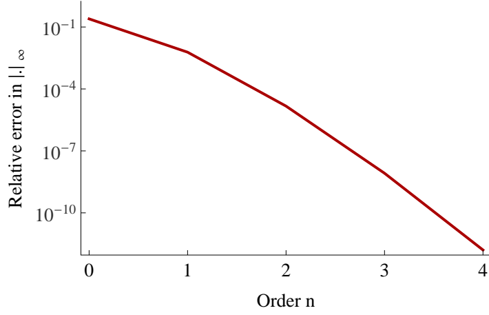
Figure 3: Relative errors in the supremum norm for problem (27) with C = 0 , a = b = \tilde{c} = \tilde{d} = 1 , c = d = \tilde{a} = \tilde{b} = 0 , \alpha = 0.775635 and \beta = 1 .
