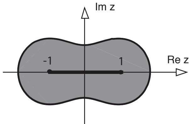
Figure 1: The Cassini disk \mathcal{D}_r = \{z \in \mathbb{C} \mid |z^2 - 1| < r\} with foci at z = \pm 1 and radius r > 1 contains the real interval [-1, 1] .
