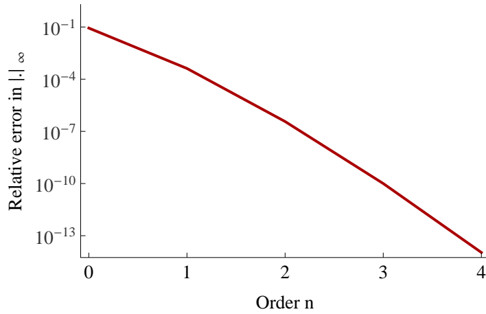
Figure 2: Relative errors in the supremum norm for problem (22) with C = 0 , a = b = \tilde{c} = \tilde{d} = 1 , c = d = \tilde{a} = \tilde{b} = 0 , \alpha = 1.94755 and \beta = 1 .
