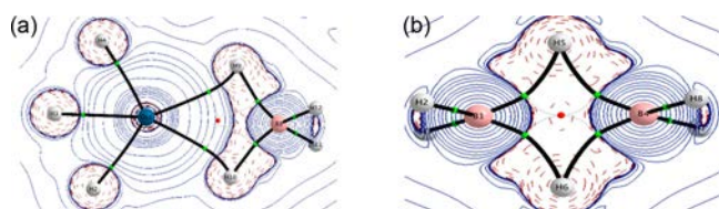
Figure 2. Contour line diagrams \nabla^2\rho(r) for (a) complex \text{OsH}_3(\kappa^2\text{-H}_2\text{BH}_2)(\text{IPr})(\text{PPh}_3) ( \text{IPr} = 1,3\text{-bis}(2,6\text{-disopropylphenyl})\text{-imidazolyli-dene} ) in the Os–H–B plane and (b) \text{B}_2\text{H}_6 in the plane of the bridging hydrogen atoms. The solid lines connecting the atomic nuclei are the bond paths, while the small green and red spheres indicate the corresponding BCPs and RCPs, respectively. [Legend: H (white), B (pink), C (gray), and Os (blue).]
