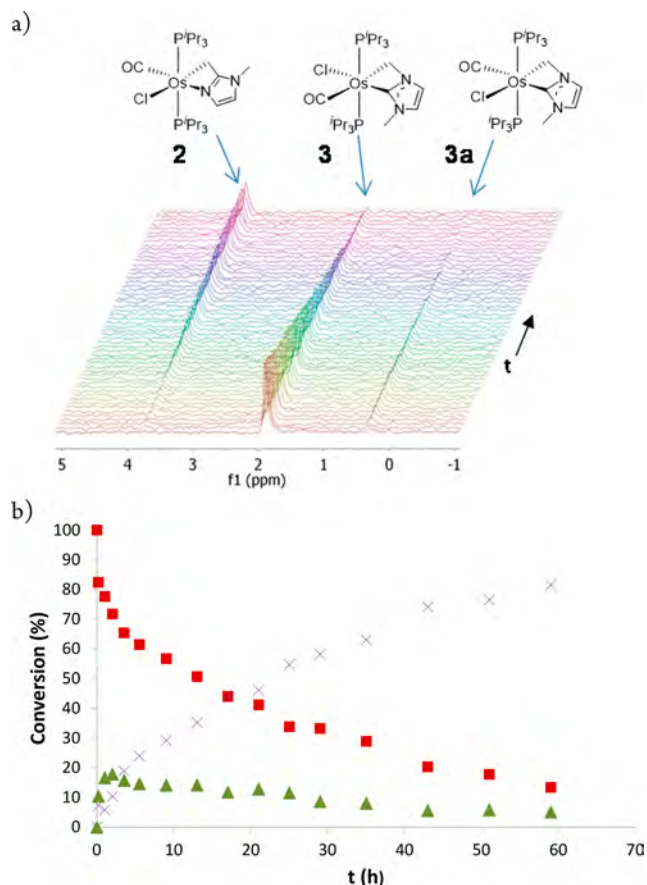
Figure 6. Transformation from 3 (red ■) to 2 (purple x) and 3a (green ▲) in toluene at 90 °C as a function of the time: (a) stacked ^{31}\text{P}\{^1\text{H}\} NMR spectra; (b) conversion versus time representation.
