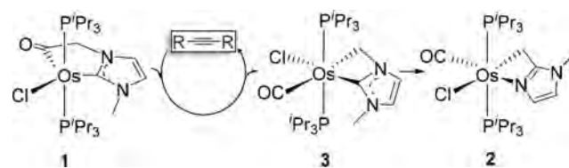
Scheme 2. Sequence of Formation of 2 and 3
