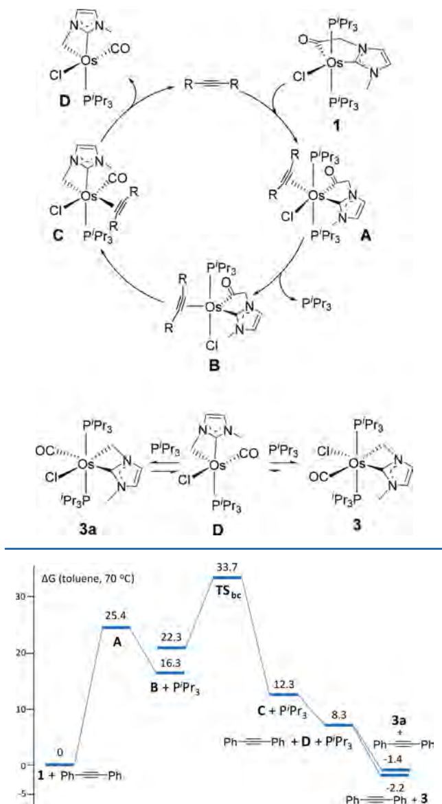
Figure 7. Energy profile ( \Delta G in \text{kcal mol}^{-1} ) of the catalysis. The energy of 1 + diphenylacetylene has been taken as a reference.
