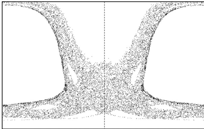
Figure 1. The plot shows a single orbit of the Poincaré map of equation (66) at \theta = 0 . The angle \phi \in [-\pi, \pi] is plotted in the horizontal axis and I_\phi \in [0, 1] in the vertical one. We have taken \epsilon = 0.8 . The energy determines I_\theta and its actual value does not affect the dynamics of \phi and I_\phi .
