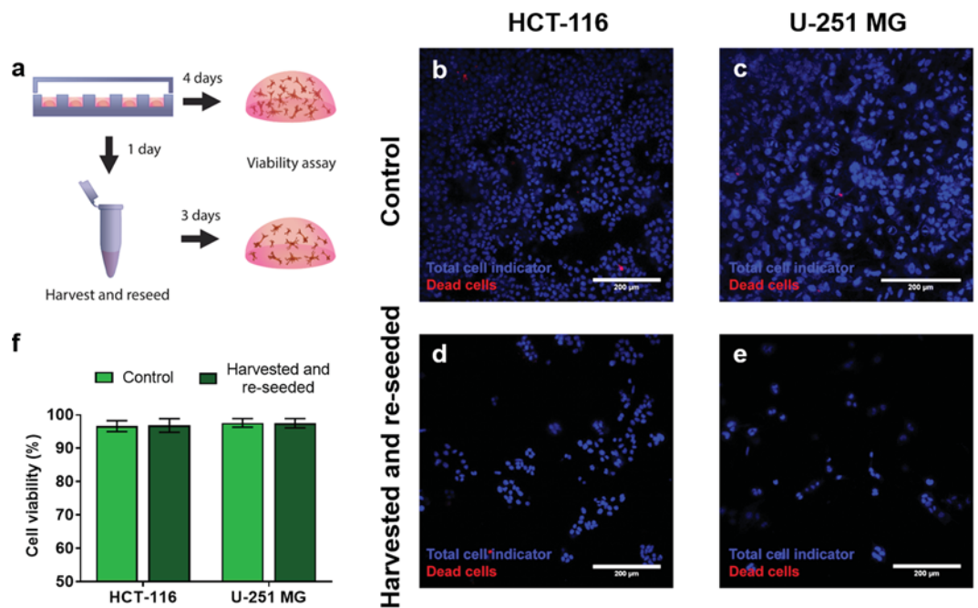
Figure 4. Biocompatibility of the cell extraction method. (a) Scheme of the experimental design. First, we embedded two different cell types independently in collagen hydrogels (HCT-116 and U-251 MG cells). After 24 hours, cells were extracted from the hydrogels by enzymatic degradation with an 8 mg/ml solution of collagenase in PBS. Recovered cells were washed with PBS and re-embedded in collagen hydrogels. Cell viability was assessed after 72 hours using confocal imaging, the cell nuclei were stained (Hoechst 33342, blue) and a dead cell indicator was added to distinguish dead cells (propidium iodide, red). Results from extracted reseeded cells were compared with non-treated cells (control). Images of the control cells can be observed in (b) for HCT-116 cells and (c) for U-251 MG cells. Images of the recovered and re-embedded cells can be observed in (d) for HCT-116 cells and (e) for U-251 MG cells. (f) Quantification of cell viability for control and extracted and re-embedded cells, for both mentioned cell types used in this study (P-value > 0.67 for HCT-116 cells and p-value > 0.99 for U-251-MG cells as determined via two-way ANOVA and post-hoc Bonferroni test).
