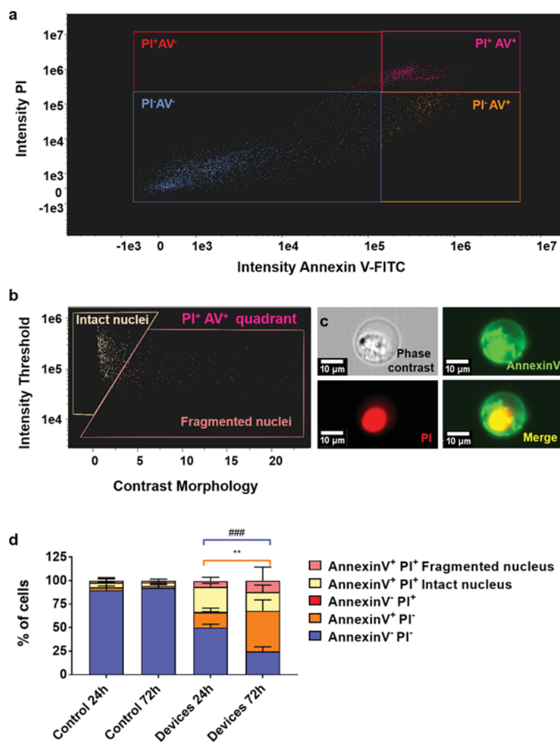
Figure 7. Validation of the degradation method for downstream AMNIS flow cytometry with individual cell imaging capabilities. (a) Sample flow cytometry 2D plot of the cell death analysis from cells extracted from a microfluidic device after 72 h of culture. (b) Breakdown of Annexin V + PI + cells from the plot shown in 7a and elucidation of their phenotype according to contrast morphology classification of nucleus integrity. (c) Single-cell sample fluorescent images of a recovered necrotic cell (Annexin V + PI + and solid nucleus in PI staining channel). Phase contrast (top-left), Annexin V-FITC (top-right), Propidium iodide (bottom-left) and merge of the two latter (bottom-right). Single-cell images were used for discerning cell phenotypes, including necrotic (intact nucleus) and apoptotic (inhomogeneous nucleus) phenotypes among Annexin V + PI + cells. (d) Graph showing the measured percentage of different cell phenotypes in the microdevices after 24 and 72 hours, according to Annexin V and PI staining and nucleus integrity for Annexin V + PI + . Controls in 2D at 24 and 72 hours are also shown to validate the staining and cell viability. Annexin V - PI - and Annexin V + PI - yielded statistically significant results after a two-way ANOVA (**p-value = 0.0011 and ###p-value = 0.0006 respectively) with a Tukey correction for multiple comparisons. Conversely, the controls were not significantly different from each other (p-value > 0.96 in all cases) and demonstrated the staining for all the described populations.
