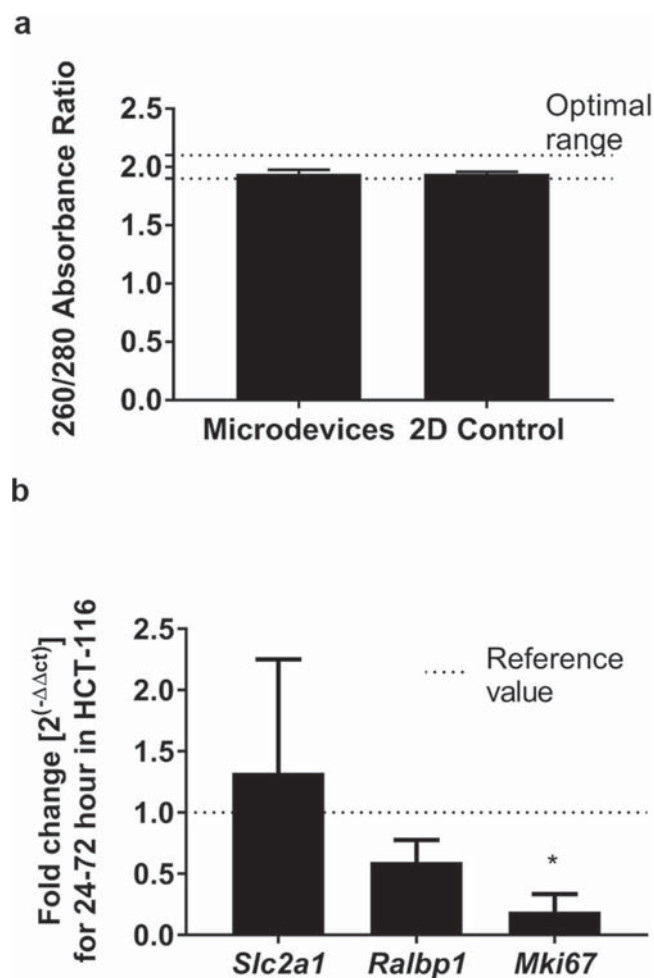
Figure 6. Validation of the degradation method for downstream qPCR. (a) 260/280 absorption ratio was determined for RNA extracted from cells seeded in 2D (2D control) and from cells seeded in microdevices. No significant differences were found (Samples passed Shapiro-Wilk normality test, and Student's t-test was performed) ( p = 0.8604 ). (b) qPCR validation of extracted RNA. Expression fold changes in Slc2a1 (Glut-1), Ralbp1 (ralA binding protein 1) and Mki67 (Ki-67) were assessed between 24 and 72 h in samples recovered from the microdevice with the described method. Actb and Gapdh were used as reference (housekeeping) genes for normalisation. Only Mki67 yielded significantly different results from the reference value (Samples passed Shapiro-Wilk normality test and were subjected to two-way ANOVA with FDR method of Benjamini, Krieger and Yekutieli) ( p = 0.012 ).
