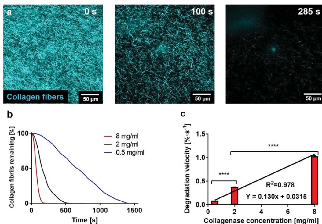
Figure 2. Optimisation of the enzymatic degradation of collagen hydrogels. (a) Confocal reflection microscopy of the degradation dynamics of a collagen hydrogel on a glass-bottomed Petri dish using an 8 mg/ml solution (18 IU/ml of collagenase P in PBS). The pictures show how the number of collagen fibrils constituting the hydrogel decreases over time. (b) Quantification of the hydrogel degradation dynamics for different collagenase concentrations through area quantification for 0.5, 2 and 8 mg/ml. (c) Characterisation of the degradation speed for the different collagenase concentrations. Linear fitting of the degradation speeds resulted in a linear equation ( Y = 0.130x + 0.0315 ) R^2 = 0.978 . Graph shows average \pm SEM (p-values < 0.001 in both cases).
