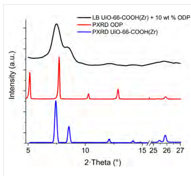
Figure 4: GIXRD pattern of an LB sample of UiO-66-COOH(Zr) + 10 wt % ODP (black line). For comparison purposes, the experimental powder diffraction of UiO-66-COOH(Zr) (PXRD, blue line) and ODP (PXRD, red line) is included.
