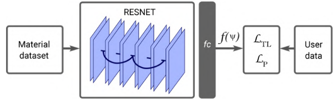
Fig. 4. Scheme of the training process, using both image data from our material dataset, and human data of perceived similarity. We train our model so that, for an input image \psi , it yields a 128-dimensional feature vector f(\psi) .
