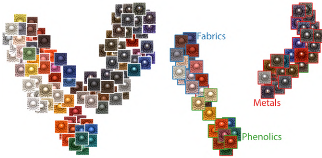
Fig. 10. Visualization of the MERL dataset in a 2D space based on the feature vectors provided by our model, using UMAP [McInnes and Healy 2018]. Left: The entire MERL dataset. Right: Materials from three different categories ( metals , fabrics , and phenolics ).
