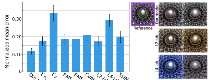
Fig. 6. Left: Mean error for different metrics (each normalized by its maximum value) with respect to distances derived from human responses, across all possible pair combinations from the MERL dataset (the \mathcal{L}_{TL} and \mathcal{L}_P columns refer to the ablation studies in Table 2; please refer to the main text). Error bars correspond to a 95% confidence interval. Right: Representative example of the two most similar materials to a given reference, according to (from top to bottom): Our model, and the two perceptually-based metrics L2-lab [Sun et al. 2017], and L4-lab [Pereira and Rusinkiewicz 2012]. Our model yields less error, and captures the notion of appearance similarity better.
