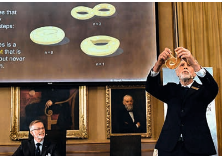
Figure 1. Torus T .
