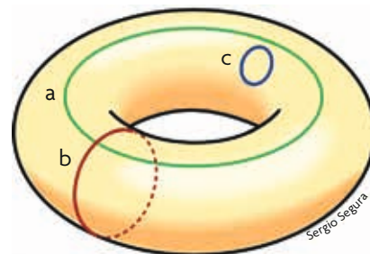
Figure 1. Torus T .
