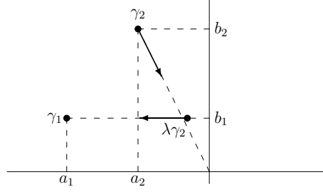
FIGURE 1. Constructing K_1 \in \mathcal{S}_0^n such that \tilde{f}_{K_1,L}(\gamma_1) = 0 .
