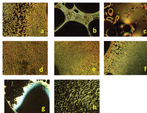
Fig. 5 POM textures of: (a) b-PEI-(1,2,4-OXA 4 ) n (taken at 179 ^{\circ}\text{C} in the 2 nd cooling), (b) l-PEI-(1,2,4-OXA 4 ) n (taken at 152 ^{\circ}\text{C} in the 1 st heating), (c) l-PEI-(1,2,4-OXA 4 ) n (taken at 222 ^{\circ}\text{C} , in the 1 st cooling), (d) b-PEI-(1,2,4-OXA 10 ) n (taken at 229 ^{\circ}\text{C} in the 1 st heating), (e) b-PEI-(1,3,4-OXA 4 ) n (taken at 170 ^{\circ}\text{C} in the 2 nd cooling), (f) b-PEI-(1,3,4-OXA 10 ) n (taken at 155 ^{\circ}\text{C} in the 2 nd cooling), (g) l-PEI-(1,3,4-OXA 4 ) n (taken at 163 ^{\circ}\text{C} , in the 1 st cooling), (h) l-PEI-(1,3,4-OXA 4 ) n (taken at 105 ^{\circ}\text{C} in the 2 nd heating).
