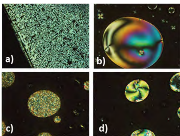
Fig. 4 POM textures of (a) 1,2,4-OXA 4 (taken at 215 ^{\circ}\text{C} in the 1 st cooling), (b) 1,2,4-OXA 10 (taken at 191 ^{\circ}\text{C} , in the 1 st cooling), (c) 1,3,4-OXA 4 (taken at 160 ^{\circ}\text{C} in the 4 th cooling), and (d) 1,3,4-OXA 4 (nematic droplets taken at 160 ^{\circ}\text{C} in the 1 st cooling).
