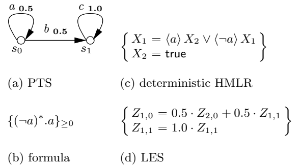
Fig. 4: Unreachable path suffix
