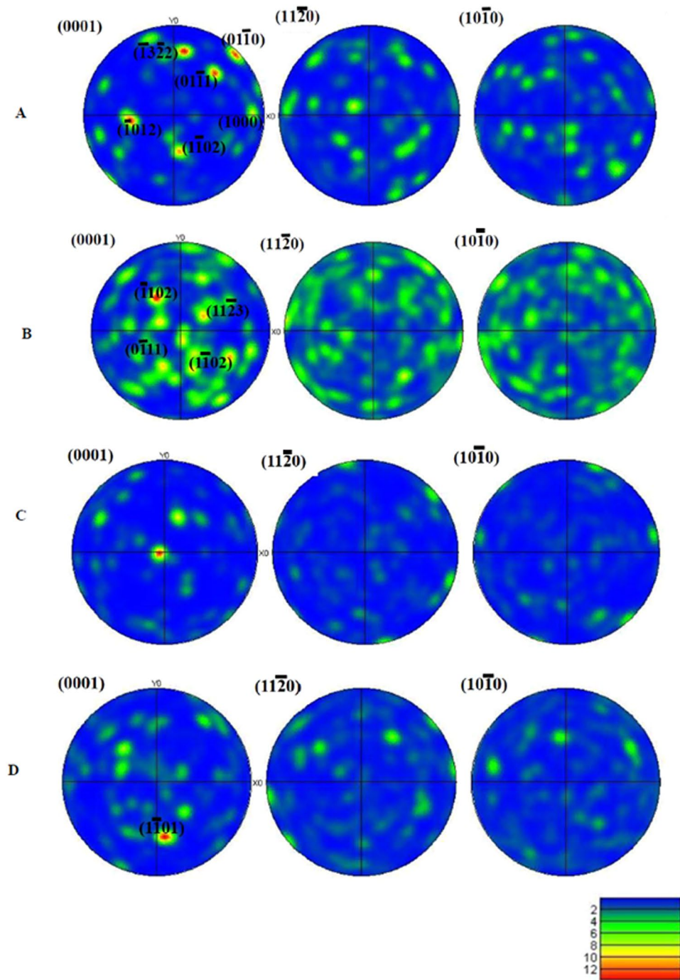
Figure 5. Pole figures of the different samples considered in this study (labelled from A to D). The (hkil) indexes of poles with a high density are provided in the (0001) stereogram.
