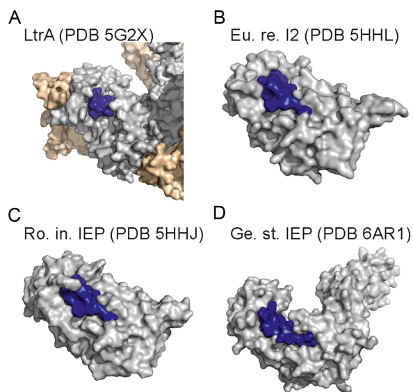
Figure 5. Overall structure representation of IEPs. (A) LtrA (PDB 5G2X). (B) Eu.re.I2. (C) Ro.in.IEP. (D) Ge.st.IEP. The surface of the IEP is depicted in grey, the QMxxxxLxxLFL motif is in blue and the intron of LtrB is in wheat colour.
