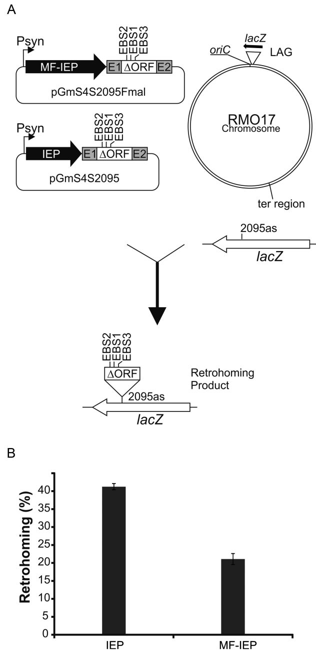
Figure 1. In vivo intron mobility assay. (A) Schematic of the assay showing intron donor plasmids (pGmS4S2095Fmal and pGmS4S2095), recipient lacZ gene and retrohoming product. LAG denotes that lagging strand DNA is used as primer for reverse transcription of the inserted intron RNA. In the lacZ gene the intron insertion site is shown (2095as). Psyn, syn promoter; EBS1,2,3, exon binding sites modified to recognize target 2095as into lacZ gene; E1, E2 short exons -20/+5 ; MF-IEP (MBP-Flag-IEP protein); IEP (wt IEP). (B) Comparison of retrohoming efficiencies between an intron expressing the wt IEP and the same intron expressing the MF-IEP fusion protein. Results are expressed as percentage of white colonies. Error bars are standard deviations (SDs) of three experiments.
