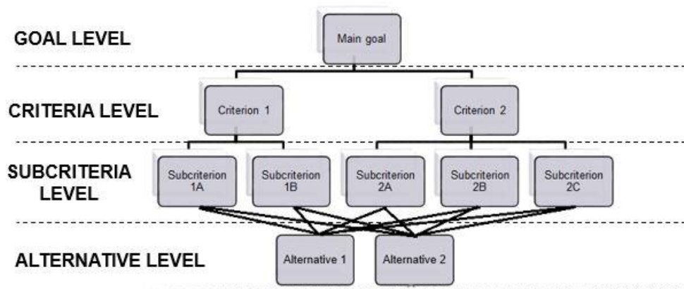
Figure 4.1: Example of AHP hierarchy
