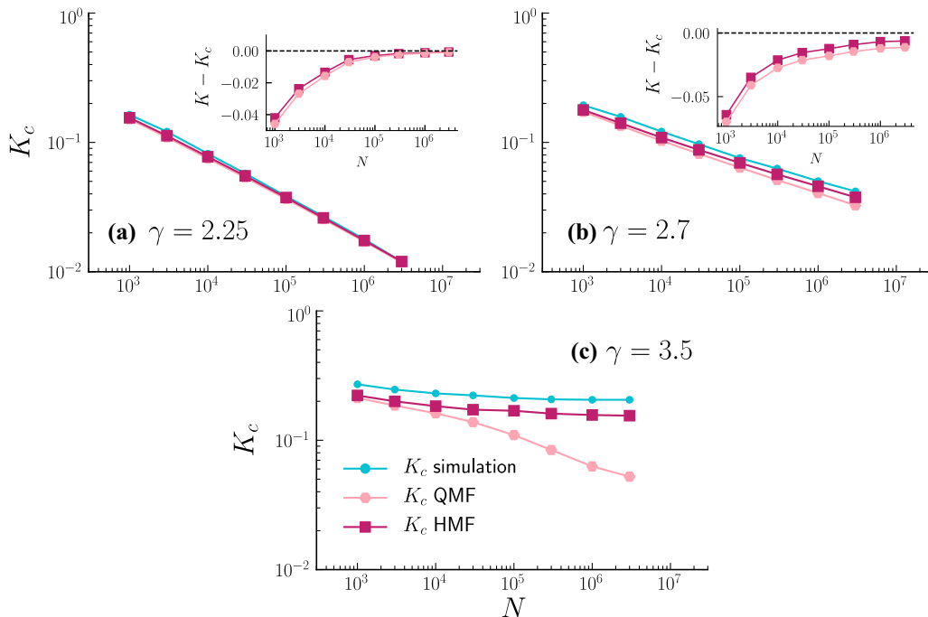
FIG. 2. Critical coupling K_c against network size N for UCM networks with power-law exponent (a) \gamma = 2.25 , (b) \gamma = 2.7 , (c) \gamma = 3.5 . All networks have k_{\min} = 5 . Insets in (a) and (b) depict the difference between numerical estimation of K_c and mean-field theories. Each point is an average over 100 network realizations. Error bars are smaller than symbols.
