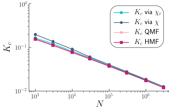
FIG. 1. Comparison between the estimations of K_c by susceptibilities \chi [Eq. (14)] and \chi_r [Eq. (15)]. Networks generated according to the UCM with degree distribution P(k) \sim k^{-\gamma} , with \gamma = 2.25 and k_{\min} = 5 . Natural frequencies are assigned according to Eq. (13). Each point is an average over 100 network realizations. Error bars are smaller than symbols.
