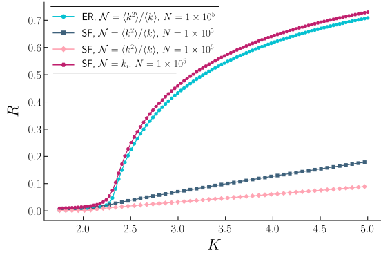
FIG. 4. Synchronization curves considering different normalizations and network topologies. Natural frequencies distributed according to g(\omega) = 1/\pi(\omega^2 + 1) . SF networks considered in this figure have \gamma = 2.25 and k_{\min} = 5 . ER were generated with the same average degree as the SF networks with N = 1 \times 10^5 . Each point is an average over 100 network realizations. Error bars are smaller than symbols.
