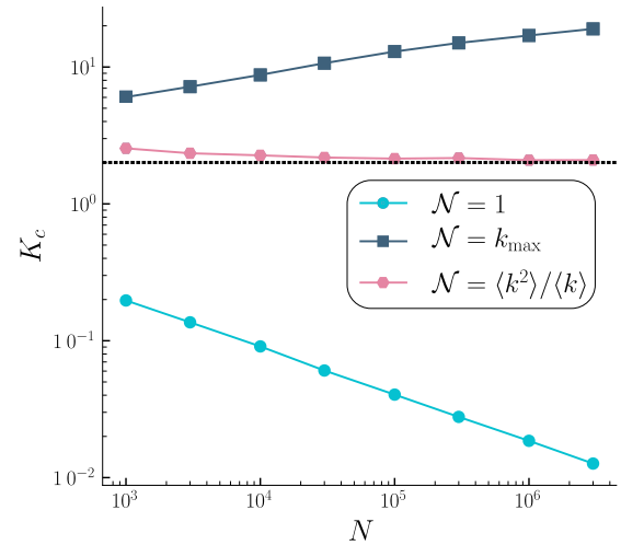
FIG. 3. Numerical calculation of critical coupling K_c as a function of number of oscillators N of SF networks with \gamma = 2.25 under different normalizations \mathcal{N} . Dashed line marks the result K_c = 2/[\pi g(0)] . Natural frequencies distributed according to g(\omega) = 1/\pi(\omega^2 + 1) . Each point is an average over 100 network realizations. Error bars are smaller than symbols.
