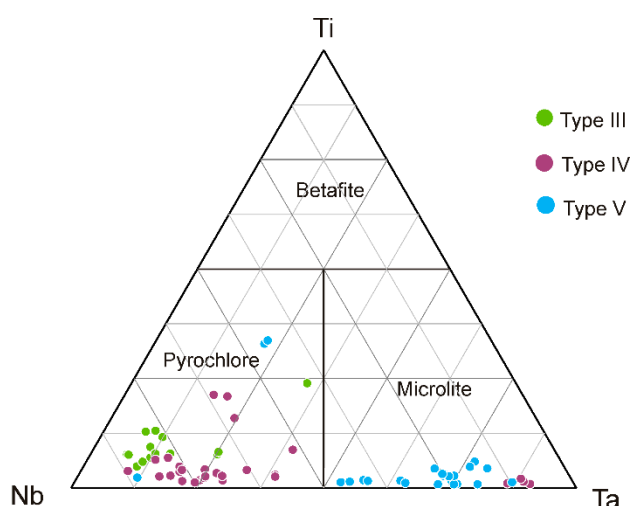
Figure 19. Nb-Ta-Ti compositional plot of the pyrochlore-super group minerals from the Giraúl pegmatites. Black solid lines after [45].
