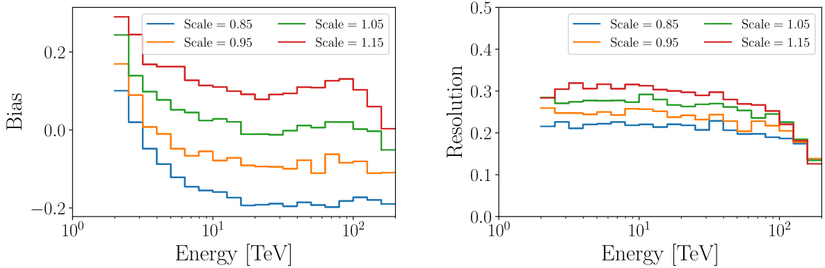
Fig. B.6. Left: bias in the VLZA energy estimation computed for different scaling values of the MAGIC light throughput system. It is estimated as the mean of the Gaussian distribution of the estimated MC energies and is given relative to the assumed true energy in the simulation. Right: VLZA relative energy resolution for different scaling values of the MAGIC light throughput system computed as the sigma of the Gaussian distribution of the estimated MC energies.
