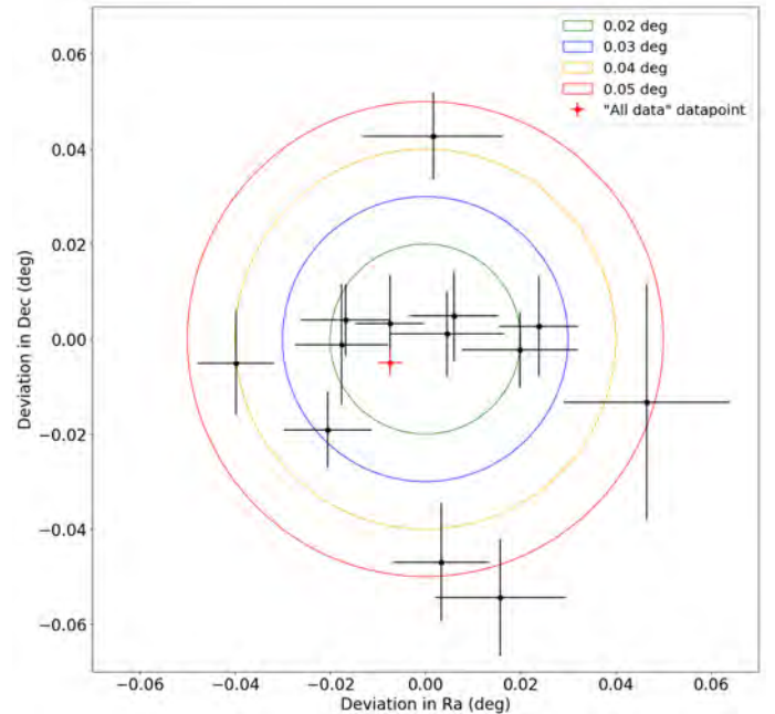
Fig. B.2. Mispointing in RA/Dec of each datapoint, as in Fig. B.1. The circles represent specific angular distances, as seen in the legend. The data point where all of the Crab VLZA data are analysed is represented in red.
