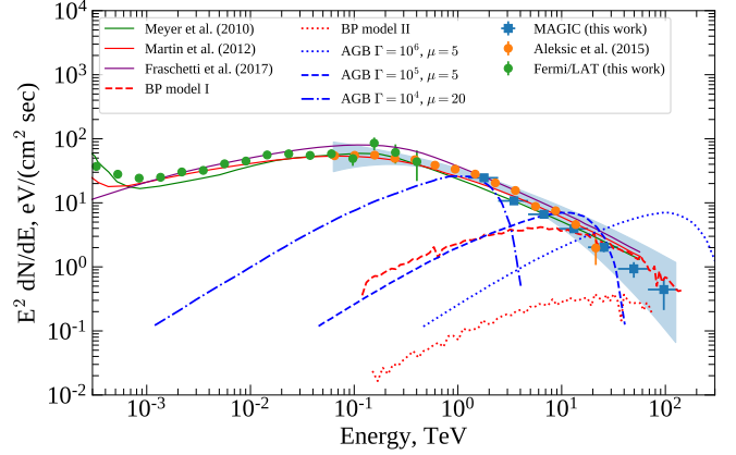
Fig. 3. Crab Nebula spectrum obtained here compared to the lower energy measurements with MAGIC (Aleksić et al. 2015) and Fermi/LAT. The blue shaded band denotes the 68% confidence flux range, estimated from the fit with the log-parabola function. Solid lines of different colours show several leptonic models from Meyer et al. (2010), Aleksić et al. (2015) and Frascchetti & Pohl (2017), previously constructed for the Crab Nebula. Dashed lines denote predictions for hadronic contribution from Bednarek & Protheroe (1997) (BP), and Amato et al. (2003) (AGB). Shown is the bulk wind Lorentz factor ( \Gamma ), and \mu = n/\bar{n} is the effective target material density increase over its mean value.
