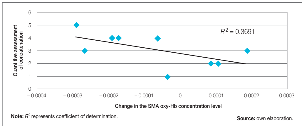
Figure 3. Correlational analysis between change in the SMA oxy-Hb concentration level due to intervention (in the in-phase condition) and the obtained concatenation score ( p = 0.08 )
