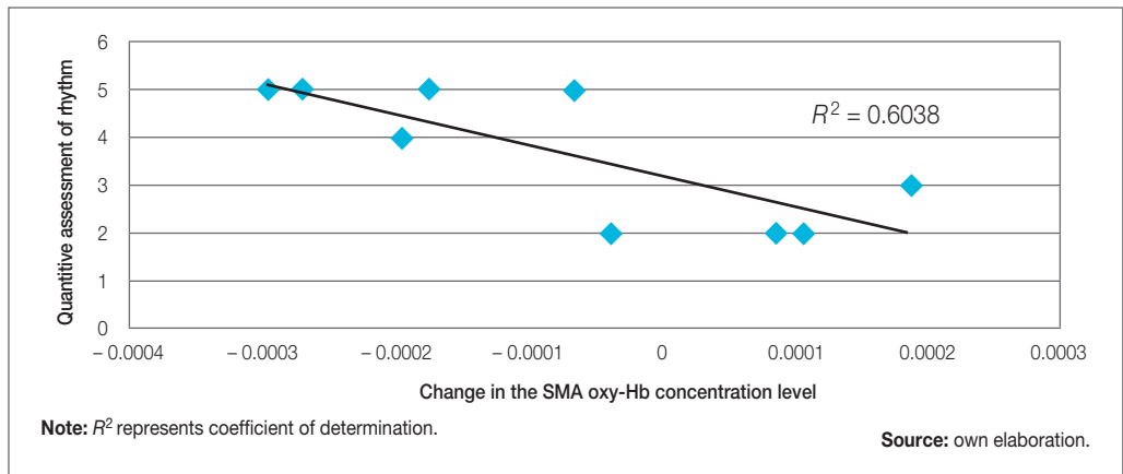
Figure 2. Negative correlation between change in the SMA oxy-Hb concentration level due to intervention (in the in-phase condition) and the obtained rhythm score ( p = 0.014 )
