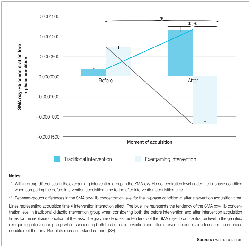
Figure 1. Between-groups and within-group differences in the SMA oxy-Hb concentration level under the in-phase condition for acquisition time
