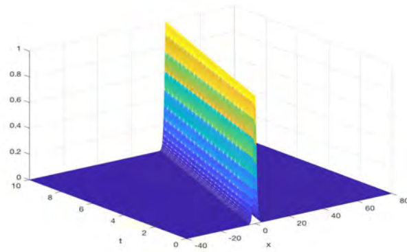
Fig. 2 Plot of u(x, t)^2 + v(x, t)^2 , solution of the NLSE problem (38)-(39).
