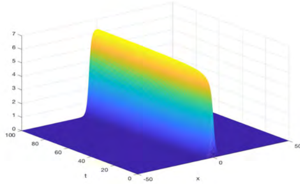
Fig. 1 Plot of u(x, t) , solution of the Sine-Gordon problem (36)-(37).
