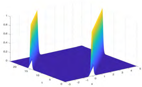
Fig. 3 Plot of u(x, t) , solution of the KdV problem (40)-(42).
