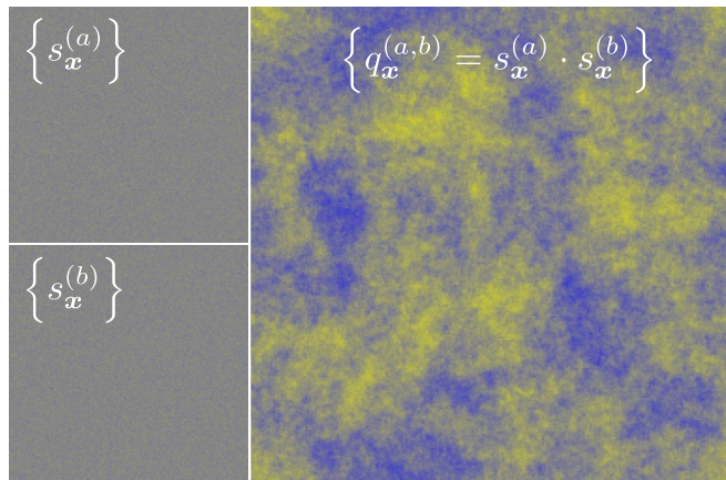
Fig. 1. Spin-glass coherence length. (Upper Left) A snapshot of a configuration \{s_x^{(a)}\} , which has evolved for t = 2^{36} Monte Carlo steps at T = 0.7 \approx 0.64T_c . We show the average magnetization on the xy plane, averaging over z . (Lower Left) Another configuration \{s_x^{(b)}\} of the same sample, prepared in the same way as \{s_x^{(a)}\} . No visible ordering is present in either configuration because the preferred pattern of the magnetic domains cannot be seen by eye ( s = 1 is plotted in yellow and -1 in blue). (Right) If one measures the overlap between the 2 configurations (Eq. 5 in Materials and Methods ) and with the same color code used for the spins, the preferred pattern of the magnetic domains, of size \xi , becomes visible. A reliable method to extract \xi from the overlap fields has been known for some time (24), but only in 2018 has it been possible to reach accuracies better than 1% in \xi (25), thanks to the Janus II computer (19) and the use of many clones for the same sample (this strategy works only if the system size, which here is L = 160 , turns out to be much larger than \xi ).
