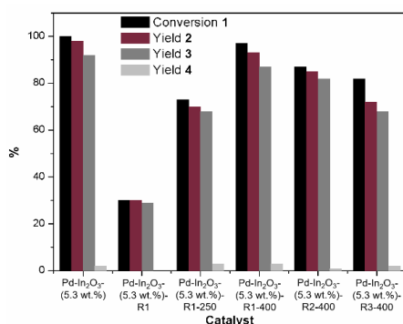
Figure 5 a) Catalyst recycling experiments for the hydrogenation of benzanilide ( 1 ). Reaction conditions: 1 (0.2 mmol), catalyst (30 mg), toluene (3.2 mL), 60 bar H 2 , 160 °C, 15 h.
