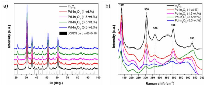
Figure 1 (a) X-ray diffraction patterns of \text{In}_2\text{O}_3 and Pd-doped \text{In}_2\text{O}_3 catalysts. The vertical lines below the XRD patterns indicate the expected reflection positions of body-centered cubic (bcc)- \text{In}_2\text{O}_3 (b) Raman spectra of \text{In}_2\text{O}_3 and Pd-doped \text{In}_2\text{O}_3 catalysts.
