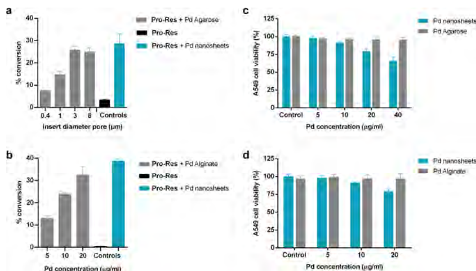
Figure 5. (a, b) Conversion of Pro-Res (100 μM) into resorufin by (a) Pd Agarose (40 μg/mL of Pd nanosheets placed in 0.4–8 μm pore size inserts) or (b) Pd Alginate (5–20 μg/mL of Pd nanosheets) after incubation in DMEM culture media (600 or 500 μL, respectively) for 16 h at 37 °C in a tissue culture incubator. Pro-Res (100 μM) with or without Pd nanosheets were used as negative and positive controls, respectively. The fluorescence signal was measured at \lambda_{\text{ex/em}} 540/590 nm. Error bars: \pm SEM from n = 3 . (c, d) A549 cell viability study after treatment with (a) Pd Agarose and (b) Pd Alginate hydrogels at different concentrations. Pd nanosheets were included as controls. Cell viability was measured at day 3. Error bars: \pm SEM from n = 3 .
