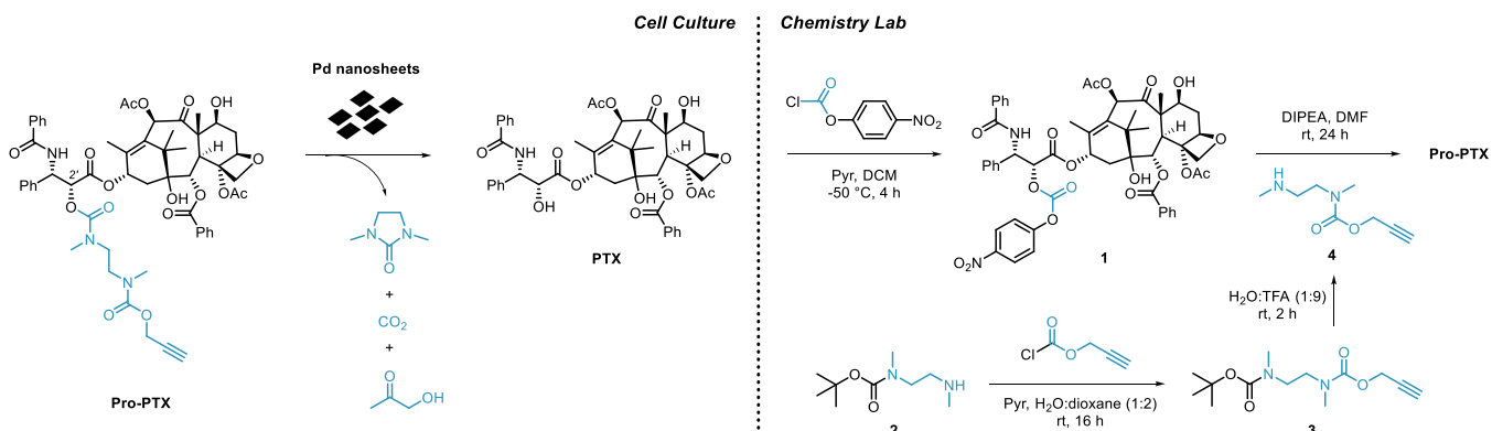
Scheme 1. Proposed Pd-Mediated Activation Strategy in Cell Culture (Left) and Synthesis of Pro-PTX (Right) a
