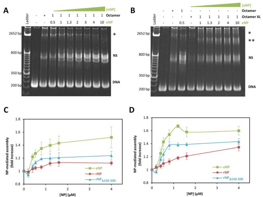
Figure 6. Nucleoplasmin (NP)-mediated transfer of histone octamers to DNA depends on chaperone post-translational modification and its C-terminal domain. 0.4 \mu M native (A) or crosslinked (B) histone octamers were incubated with increasing eNP concentrations for 1 h before the addition of 0.4 \mu M DNA. After 2 h at room temperature and 30 min at 42 ^{\circ} C, samples were analyzed by 6% native PAGE and stained with SRBR Green. The NP/Octamer molar ratio is noted above each lane. Bands marked with NS correspond to nucleosomes, and those with a single or double asterisk may be due to histone/DNA aggregates or to histone/DNA complexes generated upon transfer of crosslinked histone complexes. (C,D) NP-mediated nucleosome assembly was estimated as the intensity ratio of the nucleosome band in the presence of a given NP concentration and absence of the chaperone. Estimates are given for eNP (squares), rNP (circles; Fig. S6A,B) and rNP \Delta 150-200 (triangles; Fig. S6C,D), using native (C) or crosslinked (D) histone octamers. Lines connecting the symbols are just to guide the eye. Data are shown as mean \pm s.d. of at least three independent experiments.
