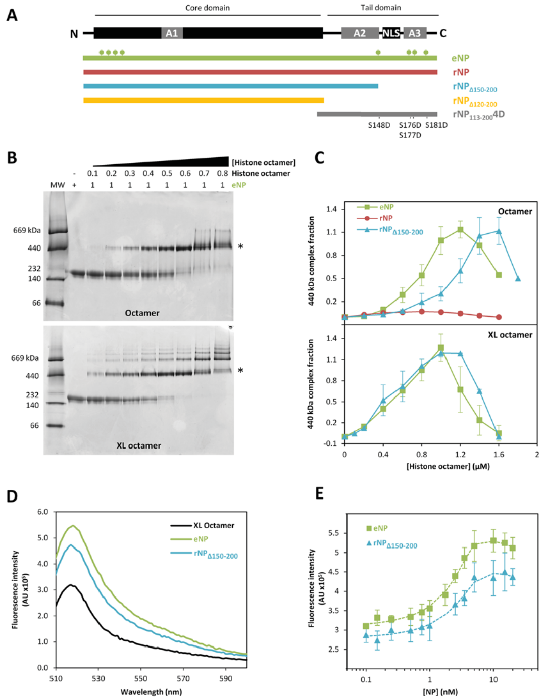
Figure 2. Phosphorylation and exposure of the acidic tract regulates nucleoplamin (NP)/histone octamer complex formation. (A) Schematic representation of the recombinant NP (rNP) variants used in this study. The phosphorylation sites (green circles) of egg NP (eNP; from X. laevis ), the position of the acidic tracts in both protein domains (A1–3), and the location of the nuclear localization sequence (NLS) are shown. (B) Titration of native histone octamers (top panel) and crosslinked octamers (XL octamer, bottom panel) with eNP. Samples were analyzed by 4–16% native PAGE and stained with Coomassie Brilliant Blue. The complex formed by two NP pentamers and a histone octamer is marked with an asterisk. (C) Quantification of the NP/octamer complex marked with an asterisk in (B) . The 440 kDa complex fraction was estimated as the ratio of the intensity of the NP/octamer complex band and that of eNP (squares), rNP (circles) or rNP _{\Delta 150-200} (triangles) in the absence of histones. Solid lines connecting the symbols have no physical meaning and are just to guide the eye. (D) Fluorescence spectra of the histone octamer (H2BT71C-Alexa 488) in the absence (black) and presence of eNP (green) or rNP _{\Delta 150-200} (blue). (E) Titration of the histone octamer (H2BT71C-Alexa488) with eNP (squares) or rNP _{\Delta 150-200} (triangles). Histone concentration was 5 nM and NP concentration is given for the pentamer. Data are shown as mean \pm s.d. of at least three different experiments. Data for rNP _{\Delta 150-200} have been shifted in the y-axis for the sake of clarity.
