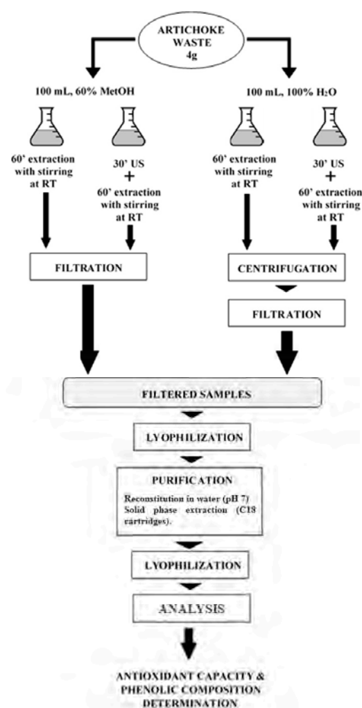
Figure 1. Diagram of the integral valorization of artichoke waste samples conducted to obtain antioxidant extracts.
