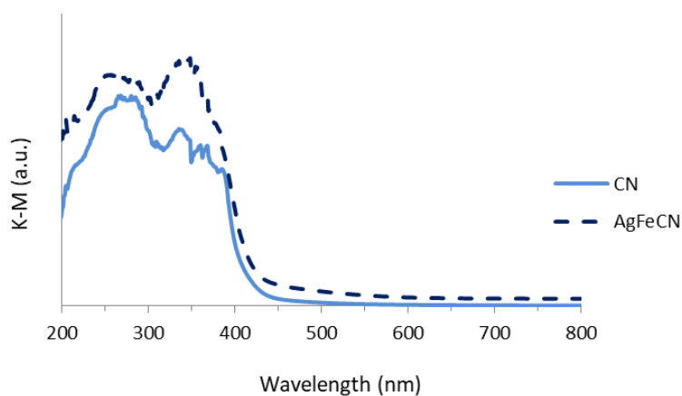
Figure 2. UV-Vis spectra of the AgFeCN composite and of pristine g-C 3 N 4 (CN).
