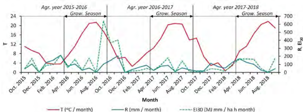
Fig. 2: Monthly values of temperature (T), rainfall depth (R), and erosivity (EI 30 ) during the test period.
