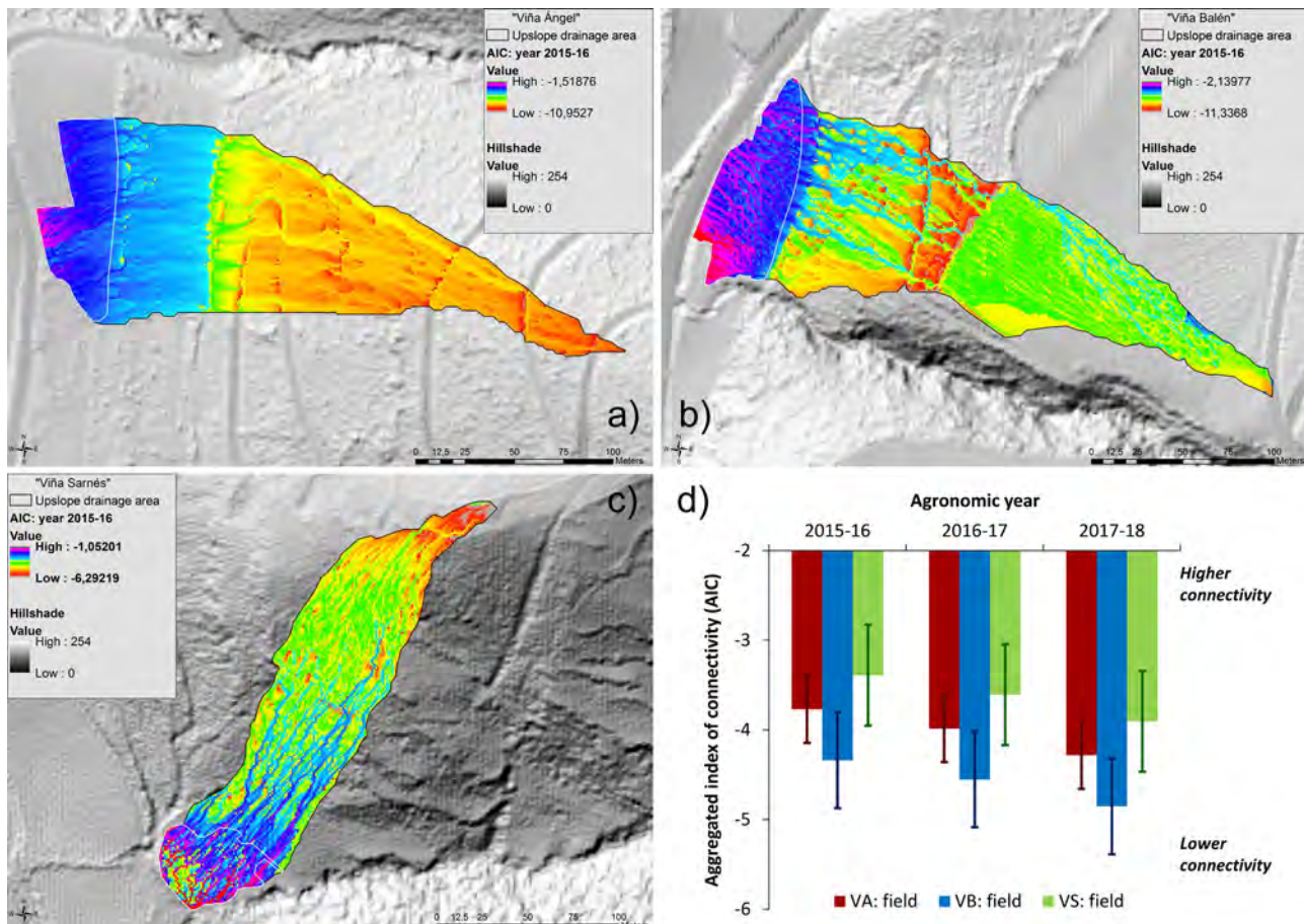
Fig. 5: Maps of runoff and sediment connectivity estimated with AIC in VA (a), VB (b), and VS (c) for the agronomic year 2015-2016. The mean and standard deviation values of AIC in the three vineyards during the test period are also shown (d).
