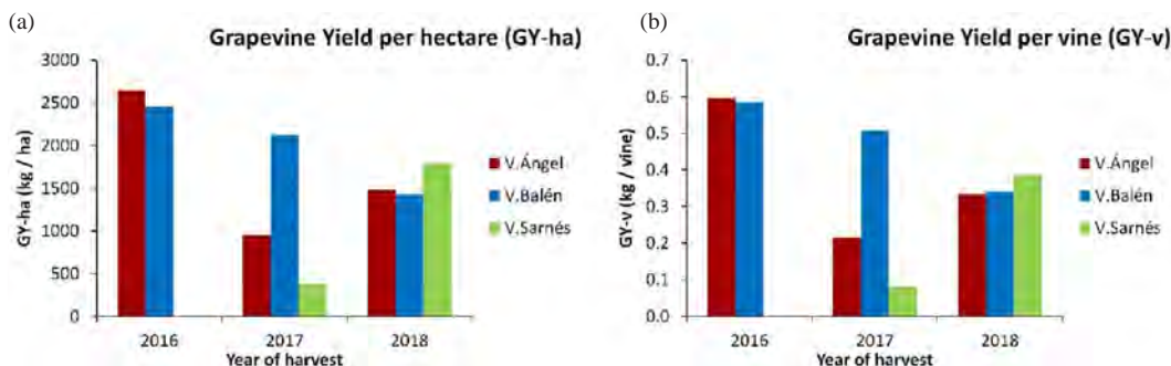
Fig. 3: Grapevine yield per ha (a) and vine (b) in the three fields and during the test period.
