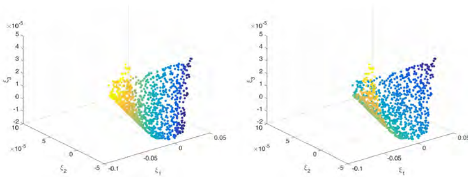
Figure 11. Reduced points colored according to the values of the coordinates h (left) and P (right).
